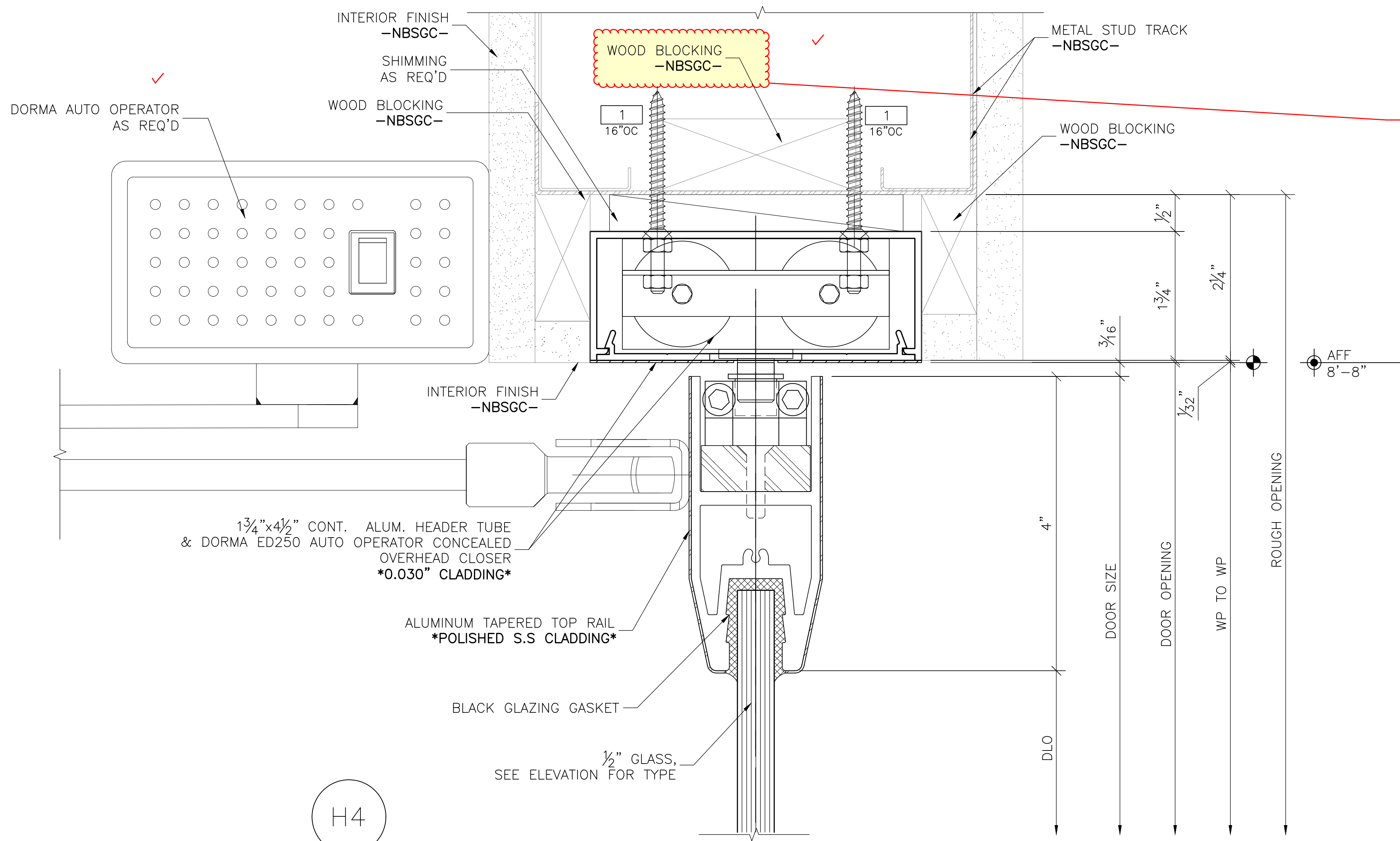
H4 DOOR HEAD DETAIL W/ CLAD TOP RAIL & HEADER TUBE COC & DORMA AUTO OP ARCH REF: NONE
