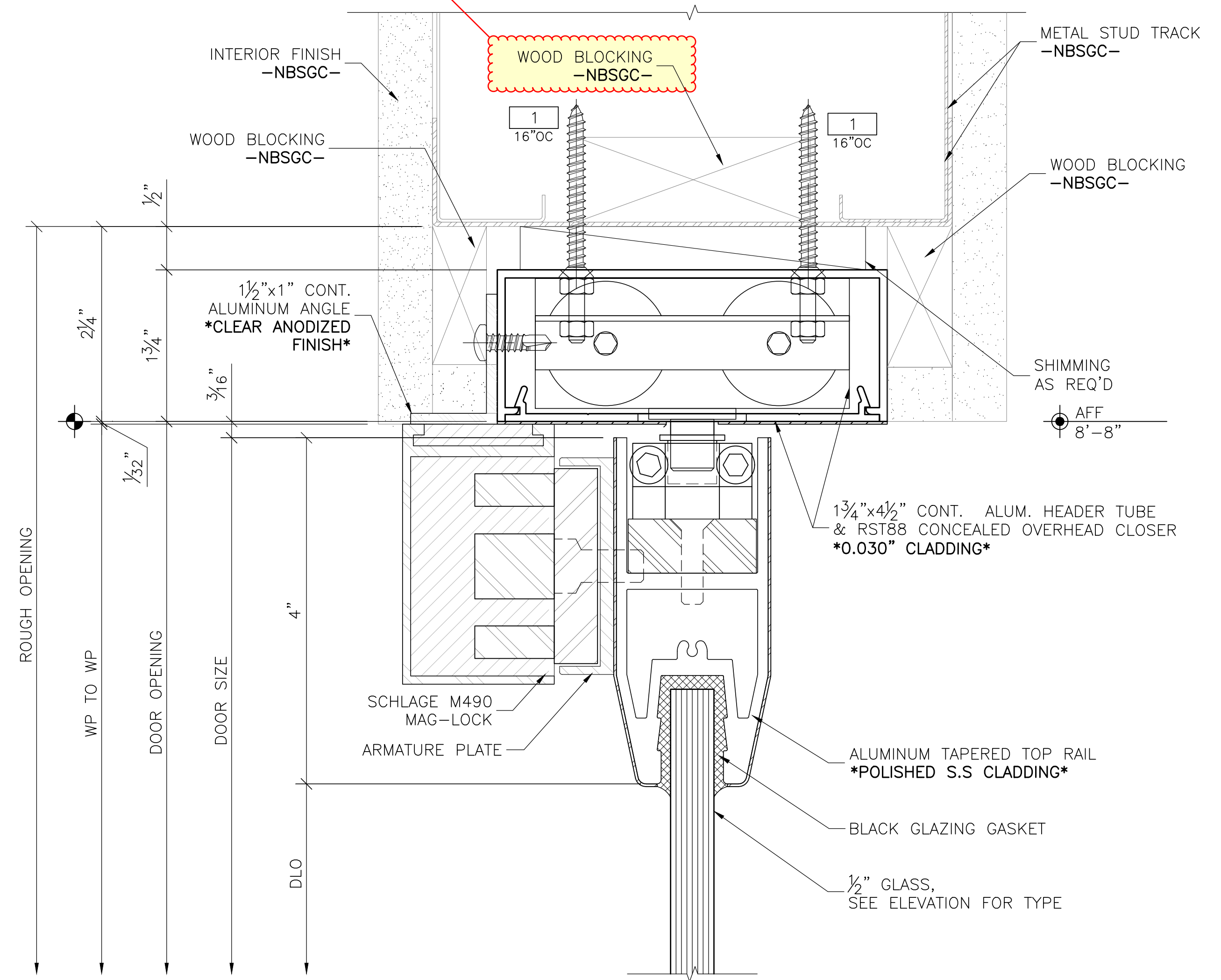
H6 DOOR HEAD DETAIL W/ CLAD TOP RAIL & HEADER TUBE COC & MAG-LOCK ARCH REF: 7/A621
